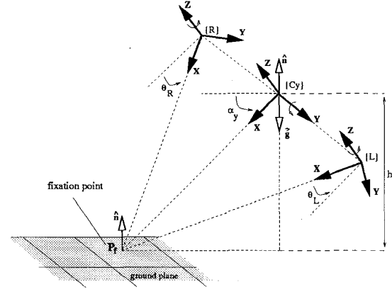
Figure 6: Ground plane point fixated. The point \vec{P}_f in the ground plane is visualised by the active vision system. The geometry of this visualisation corresponds to a state, named visual fixation.
