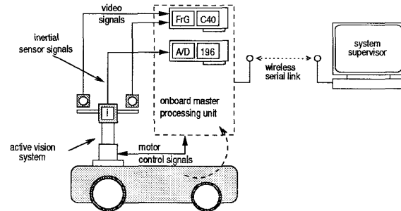
Figure 3: System Architecture. The inertial system processing board uses the Master processing unit as host computer.
