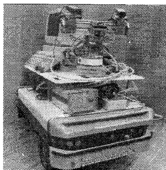
Figure 1: The mobile system with the active vision system.
