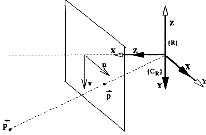
Figure 5: The camera referential and picture coordinates.
