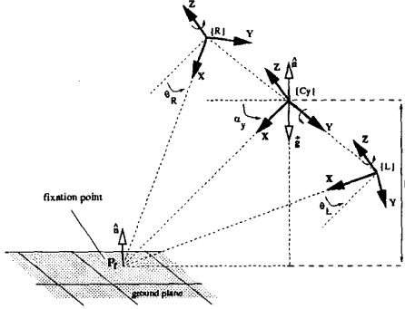
Figure 3: Ground plane point \vec{P}_f fixated.
