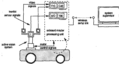
Figure 2: System Architecture.
