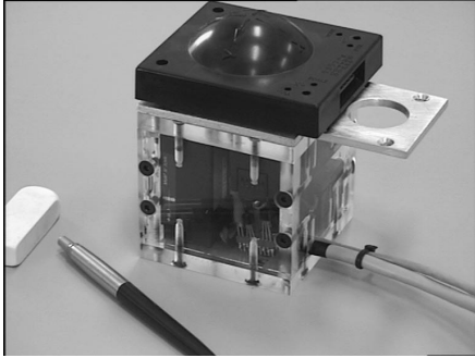
Figure 2: The inertial system prototype.
