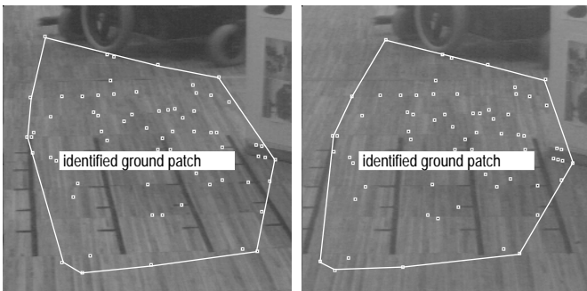
Figure 9: Identified ground patch.
