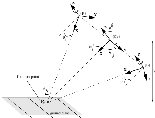
Figure 6: Ground plane point fixated. The point \vec{P}_f in the ground plane is visualised by the active vision system. The geometry of this visualisation corresponds to a state, named visual fixation.
