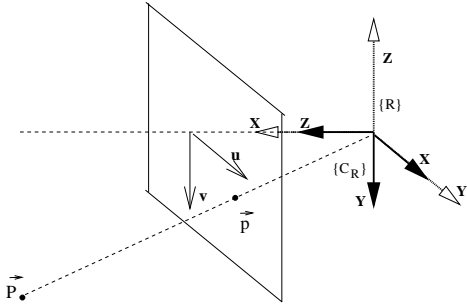
Figure 5: The camera referential and picture co-ordinates.
