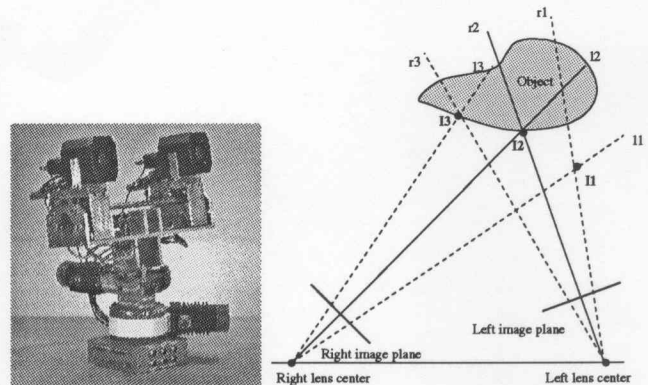
Figure 1. (a)-Active vision system (b)-Convergent cameras geometry
