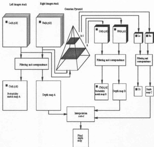
Figure 3. Algorithm overview scheme
