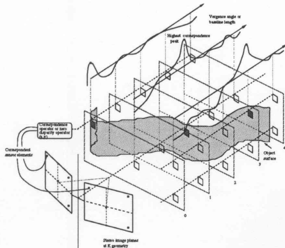
Figure 2. Space being sweep and the similarity outputs
