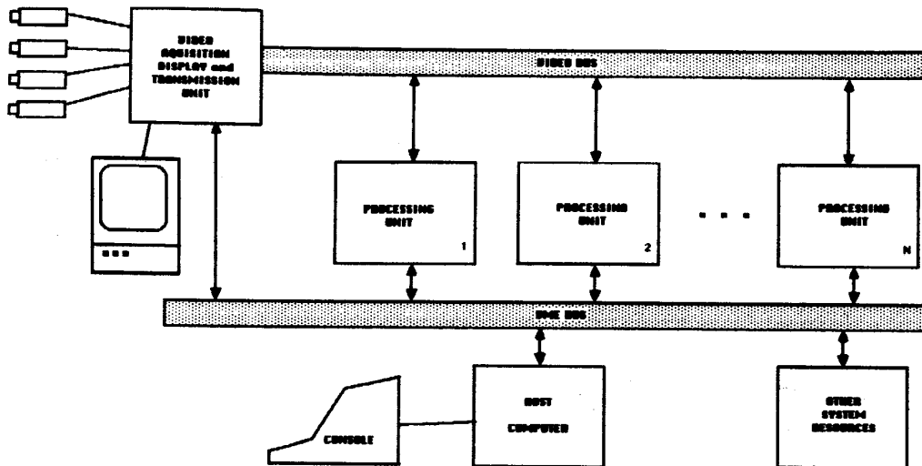
Fig.6. Vision system.
