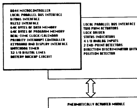
Fig. 5. Single-joint controller.
