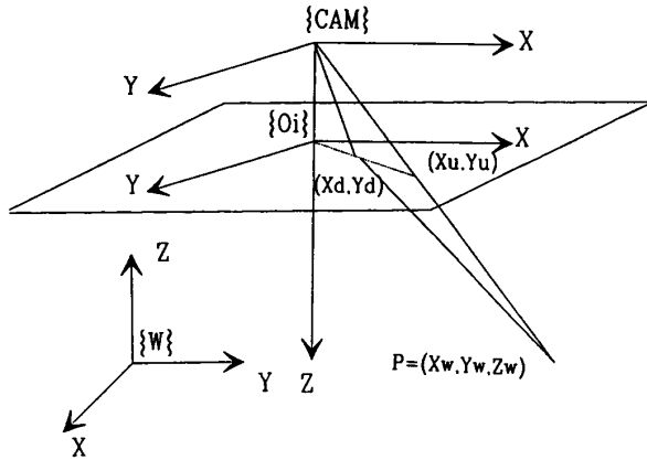
Figure 2 - The image formation model
