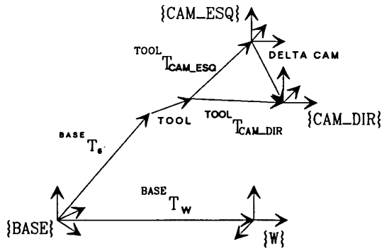
Figure 1 - Geometrical relations between the different referentials used in the system
