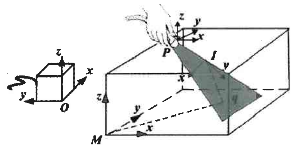
Figure 3: Coordinate Systems of the Reconstruction and Calibration Process: Image Referential (I), Position Sensor Referential (P), Transmitter Referential (O), Volume Referential (M)
