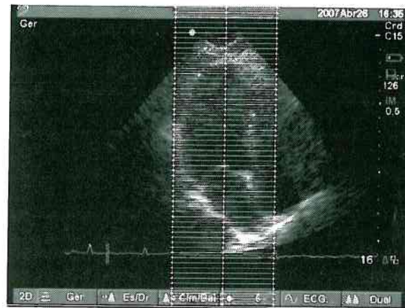
Figure 4: ROI Selection
